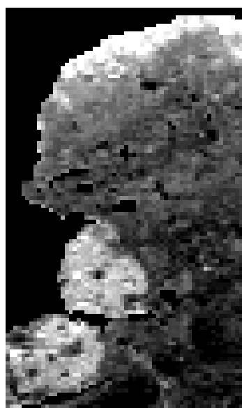
Fig. 5.11 Fraction images for arable land obtained by linear unmixing. The left fraction image is derived from the reference database LGN-2. The right fraction image is derived from the classified AVHRR image acquired on 25 July 1995.
