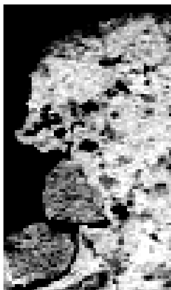
Fig. 5.8 Fraction images for grassland obtained by linear unmixing. The left fraction image is derived from the reference database LGN-2. The right fraction image is derived from the classified AVHRR image acquired on 25 July 1995.
