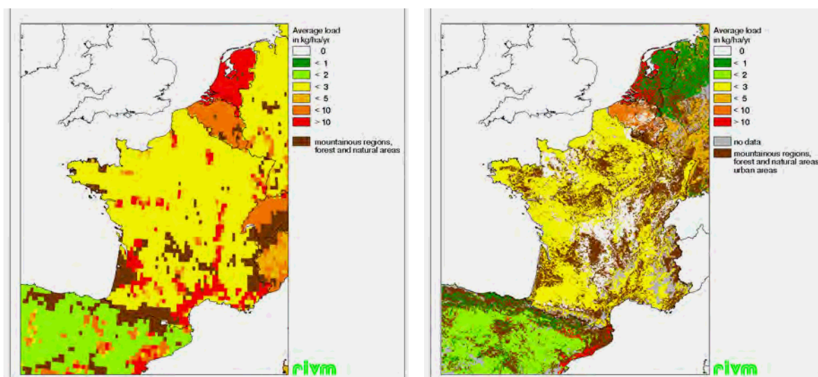
Fig. 5.4 Figure on the left shows the average pesticide load (kg /ha /year) on arable land, permanent crops and grassland using the RIVM's ten minute pan-European land use database (ELU-1). Statistics of pesticides sold per crop and per country have been obtained from Eurostat. Figure on the right shows average pesticide load (kg /ha /year) on arable land and grassland using the 1 km AVHRR-derived land cover database. Statistics of pesticides sold per crop and per country have been obtained from Eurostat.
